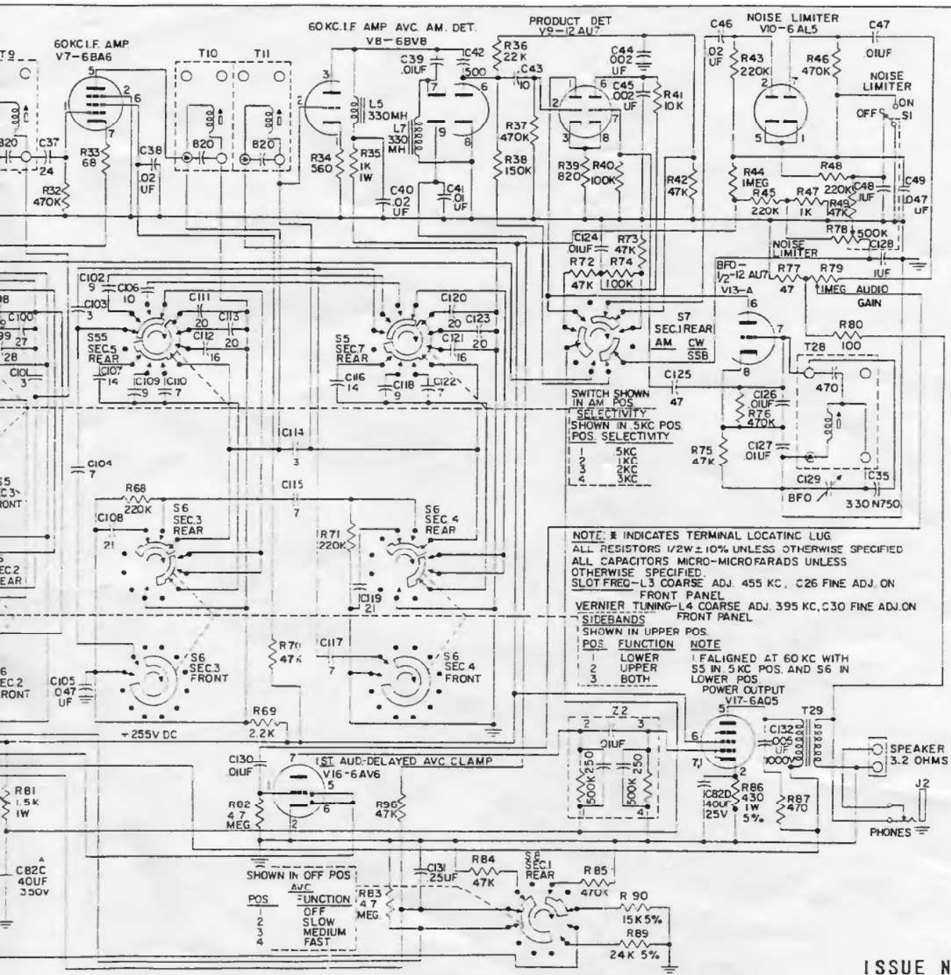
Figure 13. Hammarlund HQ-170 Communications Receiver, Schematic Diagram
